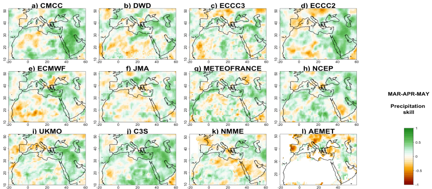
Figure 6: Precipitation correlations in MAM forecast, compared to observations, for the three seasonal forecast systems C3S (j), NMME (k) and AEMET(l). Higher values indicate better model predictive skill. From (a) to (i) models of the C3S ensemble.
