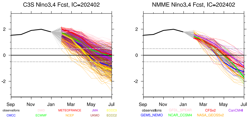
Figure 1: Niño3.4 prediction from all the ensemble members of the C3S multi-system (a) and the NMME multi-system (b), for the start-date of Fan.
