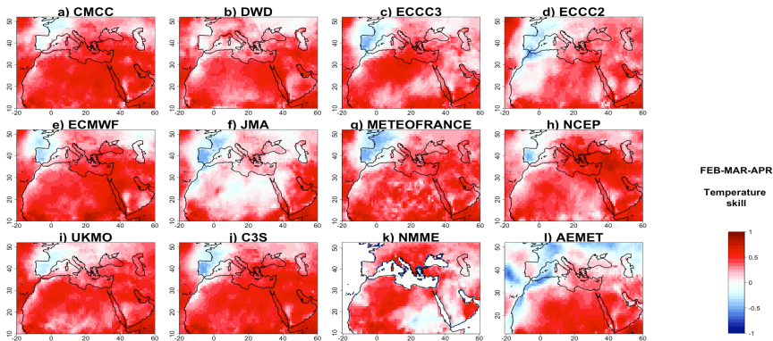
Figure 7: Temperature correlations in FMA forecast, compared to observations, for the three seasonal forecast systems C3S (j) and NMME (k) and AEMET(l). Higher values indicate better model predictive skill. From (a) to (i) models of the C3S ensemble
