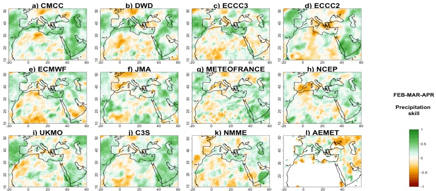
Figure 6: Precipitation correlations in FMA forecast, compared to observations, for the three seasonal forecast systems C3S (j), NMME (k) and AEMET(l). Higher values indicate better model predictive skill. From (a) to (i) models of the C3S ensemble.
