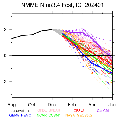
Figure 1: Niño3.4 prediction from all the ensemble members of the C3S multi-system (a) and the NMME multi-system (b), for the start-date of Jan.
