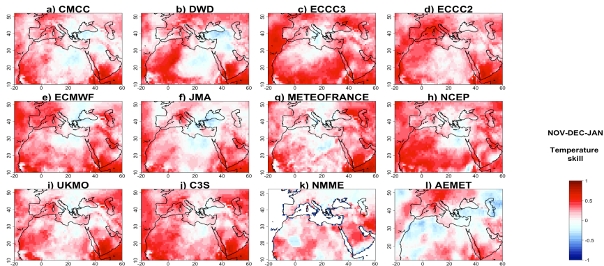
Figure 7: Temperature correlations in NDJ forecast, compared to observations, for the three seasonal forecast systems C3S (j) and NMME (k) and AEMET(l). Higher values indicate better model predictive skill. From (a) to (i) models of the C3S ensemble
