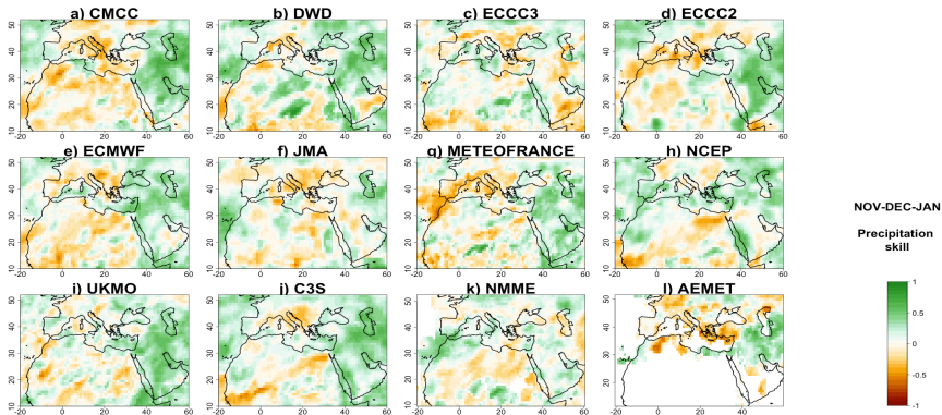
Figure 6: Precipitation correlations in NDJ forecast, compared to observations, for the three seasonal forecast systems C3S (j), NMME (k) and AEMET(l). Higher values indicate better model predictive skill. From (a) to (i) models of the C3S ensemble.
