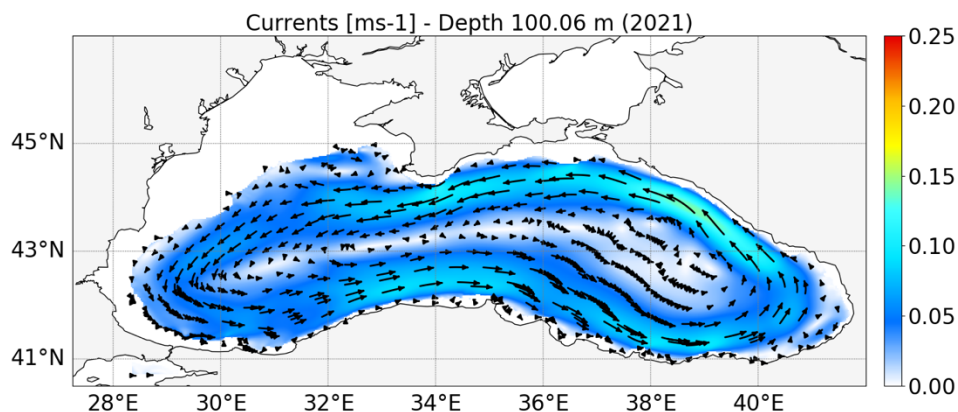
Figure 35 - 2D map of BS-PHY EAS5 circulation at ~100 m in 2021.
