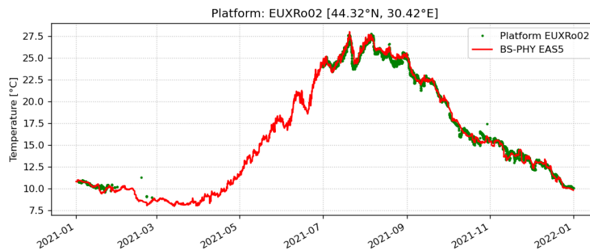
Figure 13 - CLASS2 SST comparison BS-PHY EAS5 daily analysis at hourly frequency vs EUXRo02 station observations in 2021 (T-SURF-D-CLASS2-MOOR -Jan2021-Dec2021).
