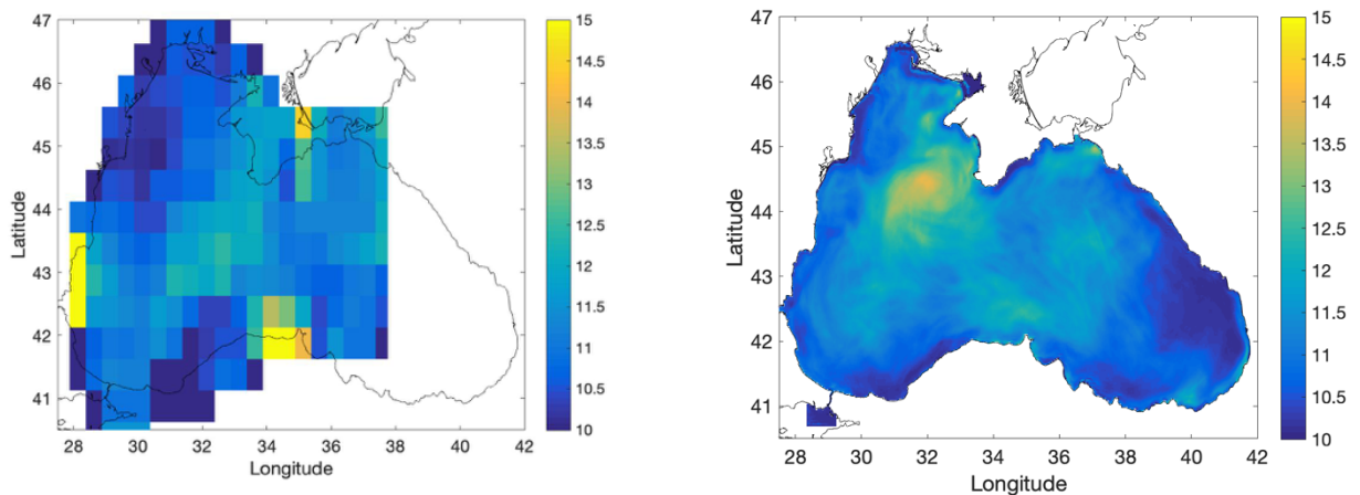
Figure 29 - Mixed layer depth values comparison May climatology from Houpert et al. (2015) (on the left) with BS-PHY EA54 May (2020-2021) (on the right).
