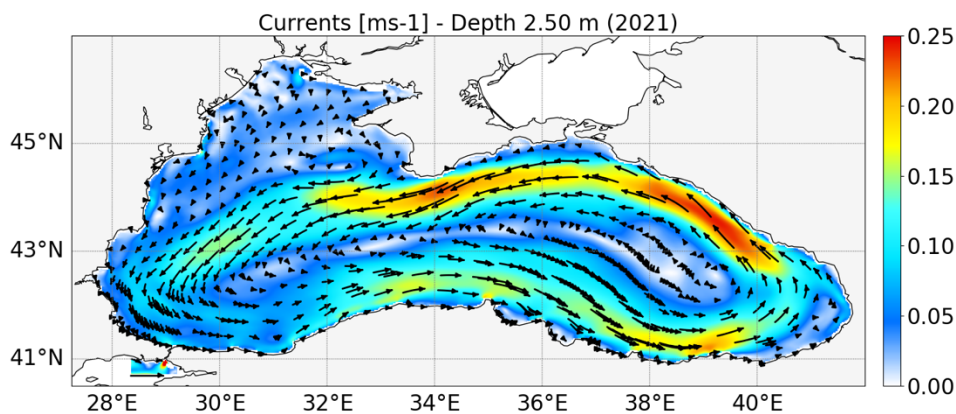
Figure 34 - 2D map of BS-PHY EAS5 circulation at surface in 2021.
