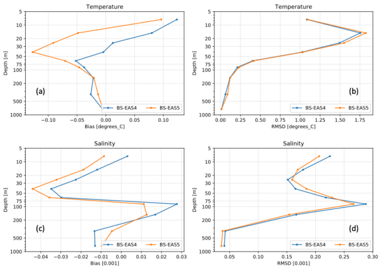
Figure 42 – EAN for temperature (bias (a) and RMSD (b)) and salinity (bias (c) and RMSD (d)) basin averaged profiles for assigned layers in 2019.
