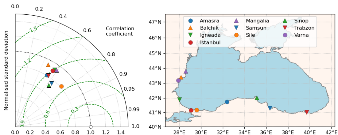
Figure 39 - Taylor diagram of the comparison between BS-PHY EAS5 and the 10 tidegauges available in the Black Sea domain for 2021. The names and locations of the tidegauges are shown on the map.
