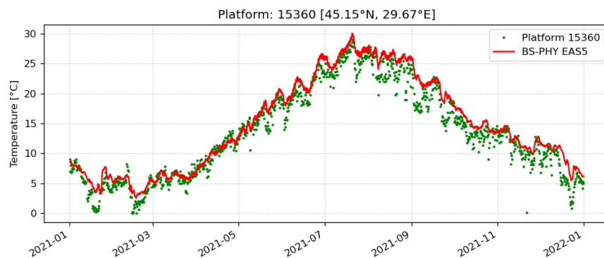
Figure 15 - CLASS2 SST comparison BS-PHY EAS5 daily analysis at hourly frequency vs 15360 station observations in 2021 (S-SURF-D-CLASS2-MOOR -Jan2021-Dec2021).
