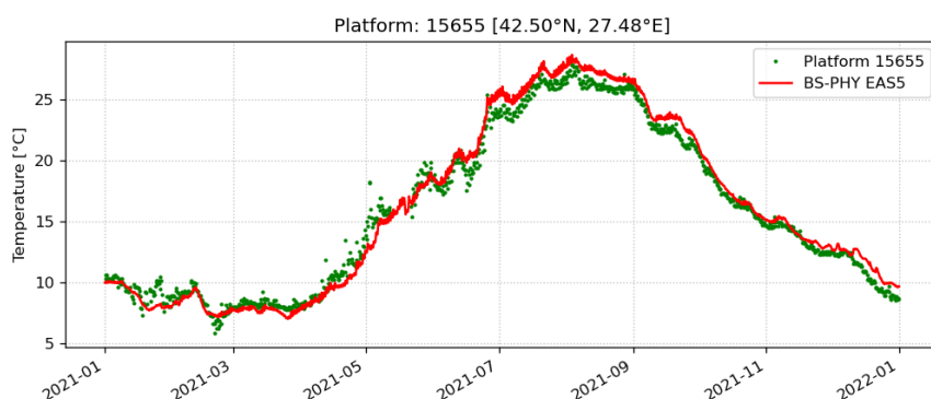
Figure 20 - CLASS2 SST comparison BS-PHY EAS5 daily analysis at hourly frequency vs 15655 station observations in 2021 (S-SURF-D-CLASS2-MOOR -Jan2021-Dec2021).
