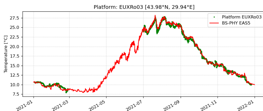
Figure 14 - CLASS2 SST comparison BS-PHY EAS5 daily analysis at hourly frequency vs EUXRo03 station observations in 2021 (T-SURF-D-CLASS2-MOOR -Jan2021-Dec2021).
