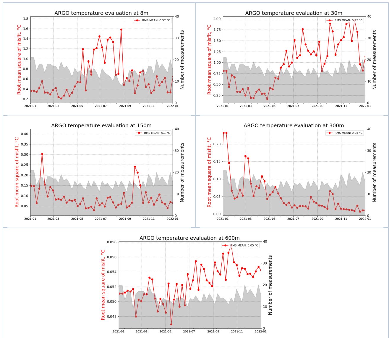
Figure 24 - Time series of weekly RMSD of temperature misfits (red solid line) and number of observed profiles (grey shaded area) at 8, 30, 150, 300 and 600 m (T-<X-Y>m-W-CLASS4-PROF-RMSD-BS-Jan2021-Dec 2021). Reference depth on top of each plot.
