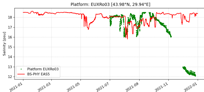
Figure 23 - CLASS2 SSS comparison BS-PHY EAS5 daily analysis at hourly frequency vs EUXRo03 station observations in 2021 (S-SURF-D-CLASS2-MOOR -Jan2021-Dec2021).
