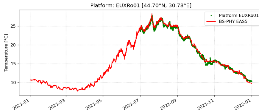
Figure 12 - CLASS2 SST comparison BS-PHY EAS5 daily analysis at hourly frequency vs EUXRo01 station observations in 2021 (T-SURF-D-CLASS2-MOOR -Jan2021-Dec2021).
