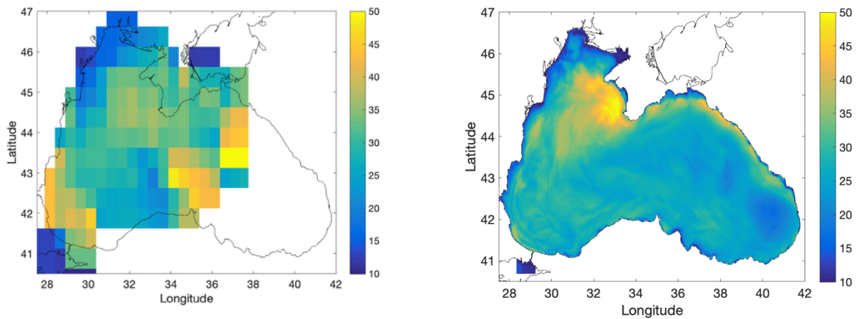
Figure 31 - Mixed layer depth values comparison December climatology from Houpert et al. (2015) (on the left) with BS-PHY EAS5 December (2020-2021) (on the right).
