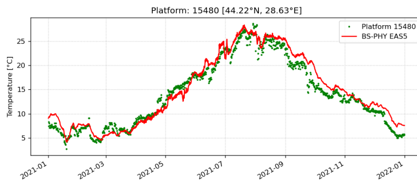
Figure 16 - CLASS2 SST comparison BS-PHY EAS5 daily analysis at hourly frequency vs 15480 station observations in 2021 (S-SURF-D-CLASS2-MOOR -Jan2021-Dec2021).
