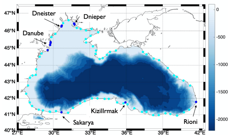
Figure 2 - Distribution of rivers in the Black Sea basin as represented in BS-NRT: minor ones are in cyan, major ones are in dark blue.
