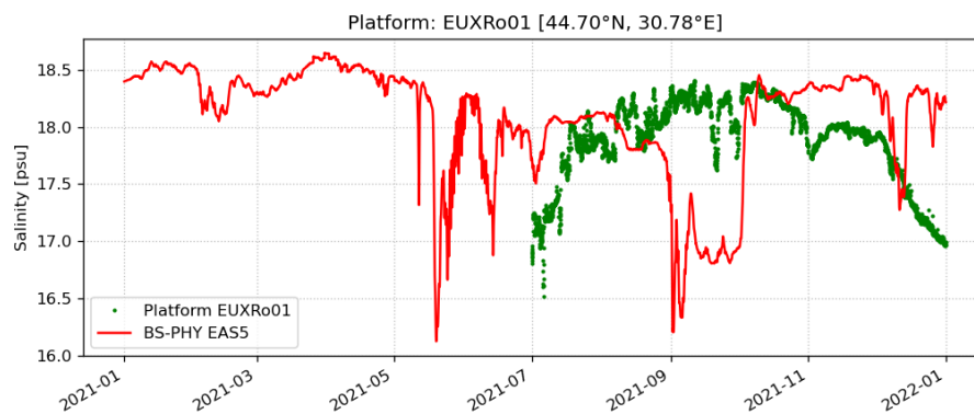
Figure 21 - CLASS2 SSS comparison BS-PHY EAS5 daily analysis at hourly frequency vs EUXRo01 station observations in 2021 (S-SURF-D-CLASS2-MOOR -Jan2021-Dec2021).
