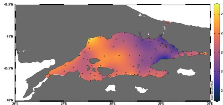
Figure 8 - U-TSS sea surface temperature (°C) 2D map and observations (black dots) in Aug 2017.
