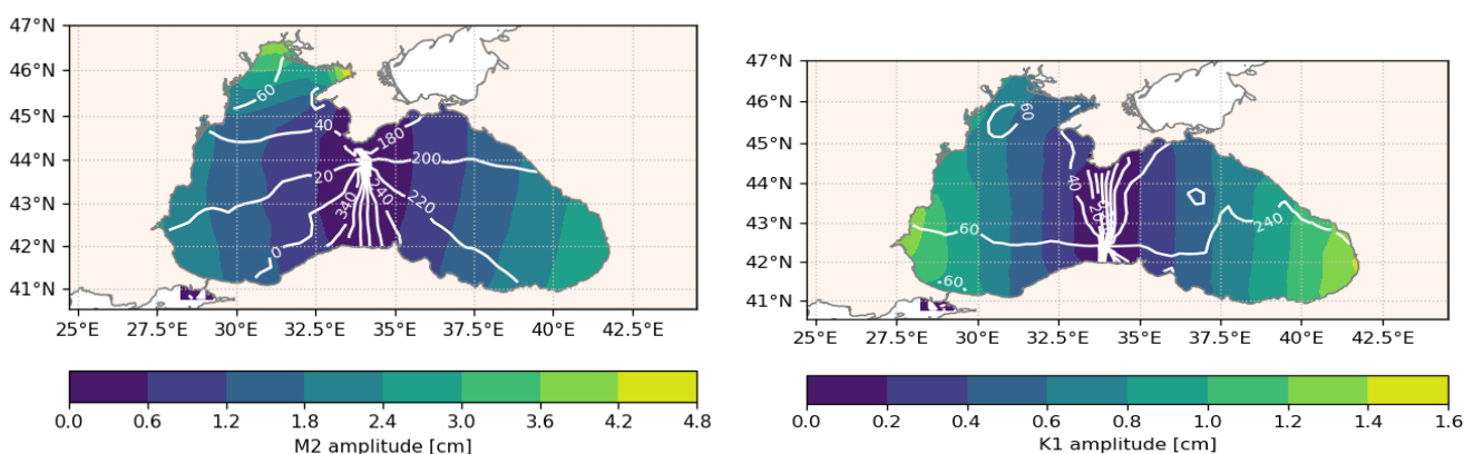
Figure 41 - Amplitude and phase of the semi-diurnal (M2, left) and diurnal (K1, right) constituents as modelled by BS-PHY EAS5. The figures can be directly compared to Fig. 4 of Ferrarin et al. (2018) and are in good agreement.
