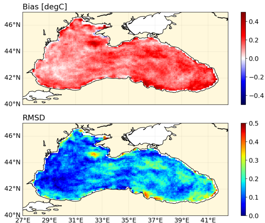
Figure 11 – 2D map BIAS (top panel) and RMSD (bottom panel) for Sea Surface Temperature using BS-PHY EAS5 analysis fields and satellite SST L3 observations on 2021.
