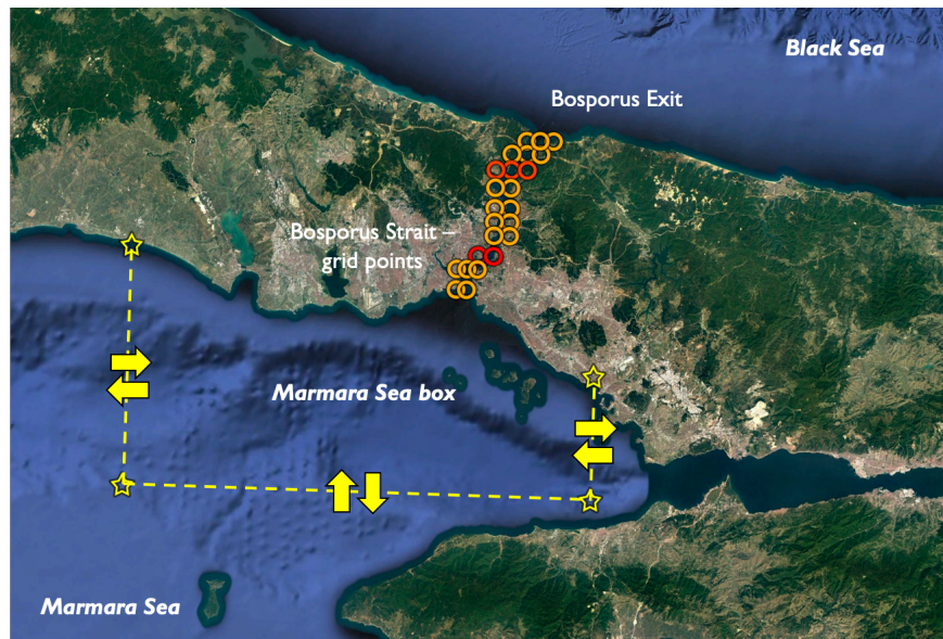
Figure 6 - Representation of the Marmara Sea box and the Bosphorus Strait in the BS-NRT.
