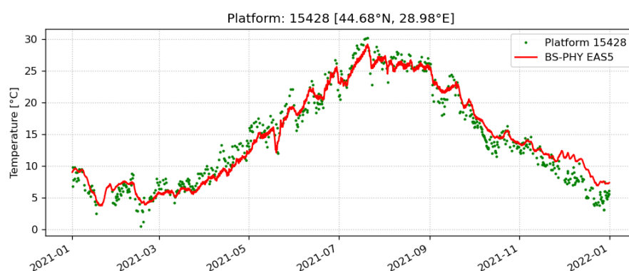
Figure 17 - CLASS2 SST comparison BS-PHY EAS5 daily analysis at hourly frequency vs 15428 station observations in 2021 (S-SURF-D-CLASS2-MOOR -Jan2021-Dec2021).
