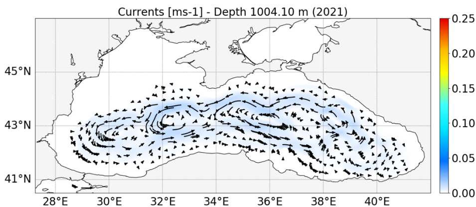
Figure 36 - 2D map of BS-PHY EAS5 circulation at ~1000 m in 2021.
