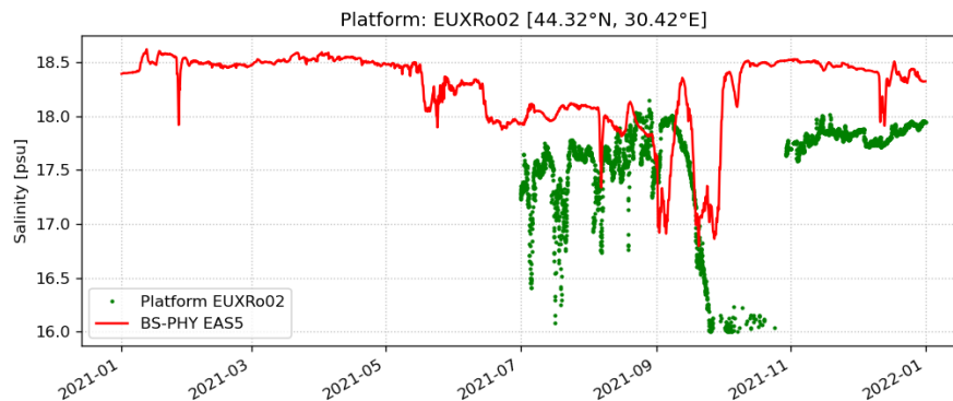
Figure 22 - CLASS2 SSS comparison BS-PHY EAS5 daily analysis at hourly frequency vs EUXRo02 station observations in 2021 (S-SURF-D-CLASS2-MOOR -Jan2021-Dec2021).
