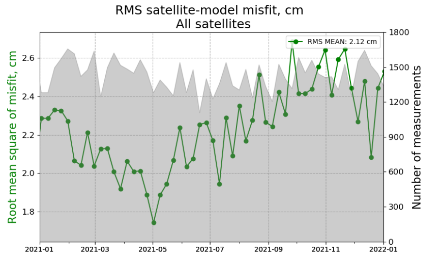
Figure 26 - Time series of weekly RMS of misfits along SLA data track for all the satellites (shaded areas in the figure) (SLA-SURF-W-CLASS4-ALL-RMSD-BS-Jan2021-Dec2021).
