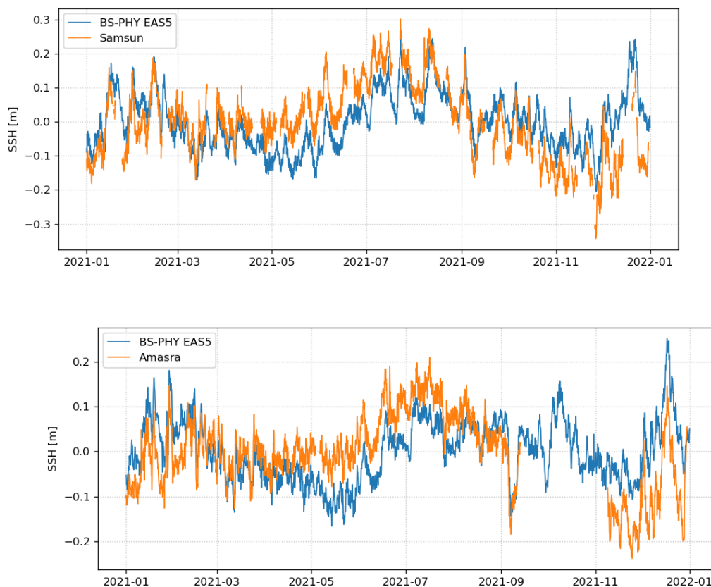
Figure 38 - Comparison of the (mean-subtracted) SSH of BS-PHY EAS5 to the tidegauges at Samsun (top) and Amasra (bottom).
