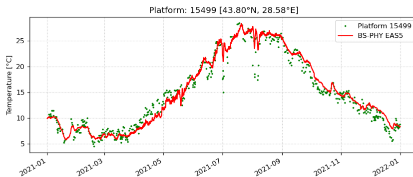
Figure 18 - CLASS2 SST comparison BS-PHY EAS5 daily analysis at hourly frequency vs 15499 station observations in 2021 (S-SURF-D-CLASS2-MOOR -Jan2021-Dec2021).
