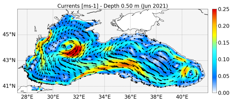
Figure 37 - 2D map of BS-PHY EAS5 circulation in June 2021.
