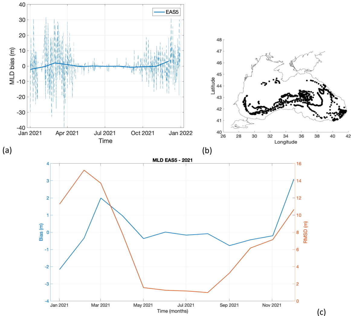
Figure 28 - a) Mixed layer depth daily and monthly bias from mode BS-EAS5 compare to ARGO floats, b) the spatial location of the floats in 2021 used in the computation of bias and RMSD, c) mixed layer bias and RMSD from model compared with ARGO floats.
