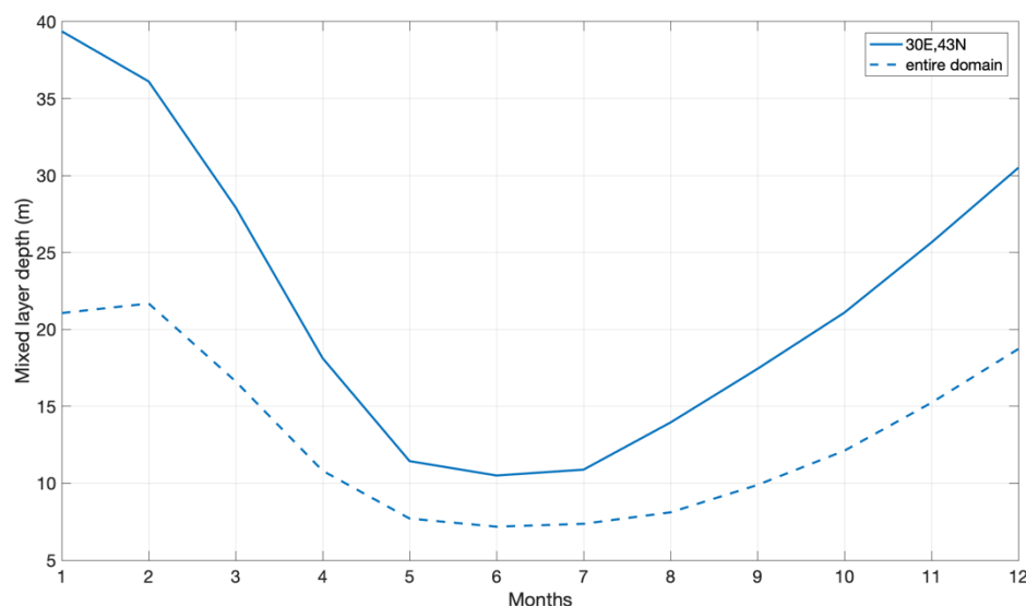
Figure 32 - Monthly mixed layer depth values in 2020-2021 at the location 43^{\circ}\text{N} , 30^{\circ}\text{E} (continuous line) and average over the entire domain (dashed line).
