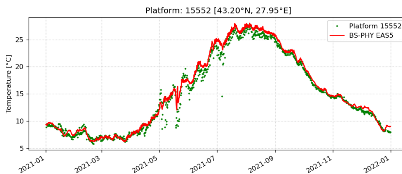
Figure 19 - CLASS2 SST comparison BS-PHY EAS5 daily analysis at hourly frequency vs 15552 station observations in 2021 (S-SURF-D-CLASS2-MOOR -Jan2021-Dec2021).
