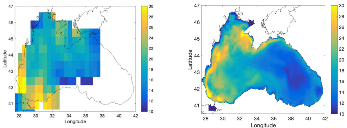
Figure 30 - Mixed layer depth values comparison October climatology from Houpert et al. (2015) (on the left) with BS-PHY EAS5 October (2020-2021) (on the right).
