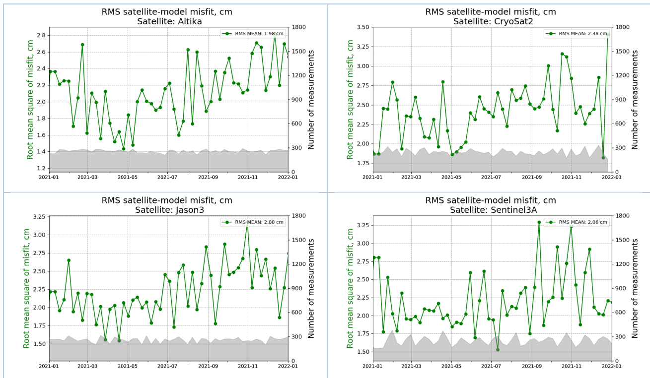
Figure 27 - Time series of weekly RMS of misfits along SLA data track from each satellites: Altika, Cryosat, Jason2, Jason3, Sentinel-3A and Sentinel-3B and corresponding number of assimilated data (shaded areas in the figures) (SLA-SURF-W-CLASS4-ALT-<PLAT>-RMSD-BS-Jan2021-Dec2021).
