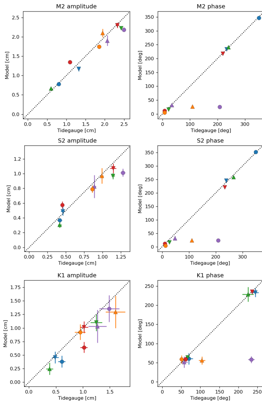
Figure 40 - Fitted amplitudes (left) and phases (right) for the main tidal constituents M2, S2 and K1. The BS-PHY EAS5 model is shown on the vertical axis and the fit obtained from the tidegauge data on the horizontal axis. The markers correspond to the stations as shown in Fig. 39.
