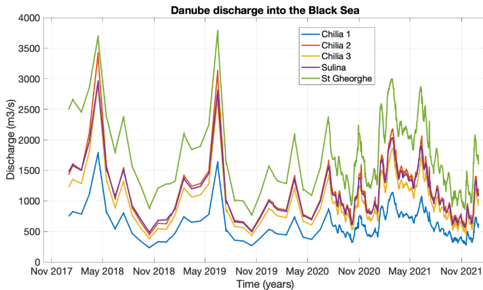
Figure 4 - Daily discharges for the Danube outlets: NIHWM interannual dataset from January 2018 until June 2020 and daily observations from July 2020 onwards as accounted in the BS-NRT model.
