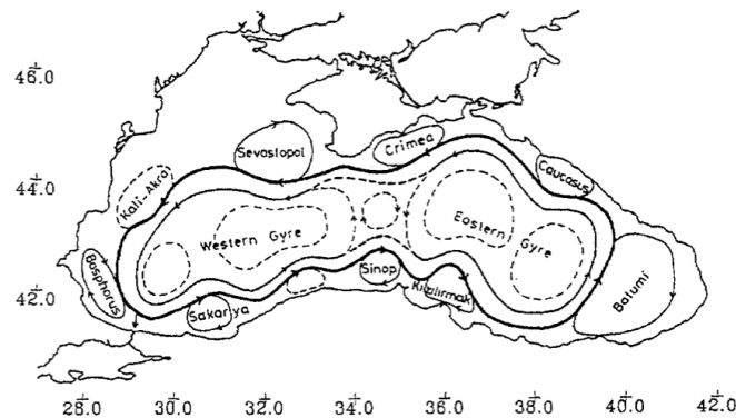
Figure 33 - General circulation of the Black Sea as proposed by Ozsoy and Unluata (1997) using the observations available until the study conducted.
